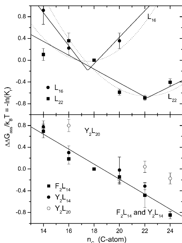
FIGURE 3 Chain length dependence of the phosphatidylcholine association constants, K_r , relative to diC(18:1)PtdCho, for association with transmembrane oligoleucine helical peptides with different lengths and different anchoring groups. The different chain length phosphatidylcholines are diC(14:1c \Delta^9 )PtdCho, diC(16:1c \Delta^9 )PtdCho, diC(18:1c \Delta^9 )PtdCho, diC(20:1c \Delta^{11} )PtdCho, diC(22:1c \Delta^{13} )PtdCho, and diC(24:1c \Delta^{15} )PtdCho. The ordinate is plotted to yield the free energy of association \Delta\Delta G_{\text{ass}}/k_B T = -\ln K_r , relative to diC(18:1)PtdCho. (Upper panel) Ac-K 2 GL 7 WL 9 K 2 A-mide ( L_{16} ) and Ac-K 2 GFL 10 WL 12 FK 2 A-mide ( L_{22} ) (data from Web et al. (59)). Error bars are given for a representative \pm 0.1 uncertainty in K_r . (Solid lines) Least squares fits of Eqn. 14 with the parameters \Delta g_{\text{mis}} and n_p that are given in Tables 1 and 2, respectively. (Dotted lines) Predictions of Eq. 9 with n = n_p . (Lower panel) Ac-K 2 GFL 6 WL 8 FK 2 A-mide ( F_2L_{14} ), Ac-K 2 GYL 6 WL 8 YK 2 A-mide ( Y_2L_{14} ), and Ac-K 2 GYL 9 WL 11 YK 2 A-mide ( Y_2L_{20} ) (data from Mall et al. (60)). (Solid line) Least-squares fit of Eq. 14, with fixed n_p = 25 , to the combined data for F_2L_{14} and Y_2L_{14} .
