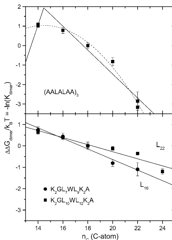
FIGURE 6 Lipid chain length dependence of the association constant for dimer formation, K_{\text{dimer}} , of transmembrane helical peptides. The phosphatidylcholine lipid hosts are diC(14:1c \Delta^9 )PtdCho, diC(16:1c \Delta^9 )PtdCho, diC(18:1c \Delta^9 )PtdCho, diC(20:1c \Delta^{11} )PtdCho, diC(22:1c \Delta^{13} )PtdCho, and diC(24:1c \Delta^{15} )PtdCho. The ordinate is plotted as the free energy of dimerization \Delta G_{\text{dimer}}/k_B T = -\ln(K_{\text{dimer}}) , and values are given relative to diC(18:1)PtdCho. (Upper panel) Ac-(AALALAA) 3 -amide antiparallel heterodimers with energy-transfer fluorophore couples at either N- or C-terminus (data from Yano and Matsuzaki (74)). Peptide is given a double weighting with respect to lipid in calculating mole fractions because it spans both halves of the bilayer. (Dotted line) Prediction of Eq. 9 with optimization of n_P = 14.5 \pm 0.6 and an adjustable multiplicative factor \Delta N_L = 1.7 \pm 0.4 . (Solid line) Least-squares fit of Eq. 14 with fixed n_P = 14.5 and the optimized value of \Delta N_L \Delta g_{\text{mis}}/k_B T given in Table 3. (Lower panel) Ac-K 2 GL 7 WL 9 K 2 A-amide (L 16 ) and Ac-K 2 GL 10 WL 12 K 2 A-amide (L 22 ) heterodimers with the corresponding quencher peptides bearing dibromotyrosine instead of tryptophan (data from Mall et al. (76)). Solid lines are least-squares fits of Eq. 14 with fixed n_P = 14 and optimized values of \Delta N_L \Delta g_{\text{mis}}/k_B T given in Table 3.
