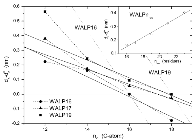
FIGURE 9 Chain length dependence of the maximal increase in hydrophobic thickness, d_c - d_c^0 , for the diC( n_c :0)PtdCho lipids directly adjacent to Fm-AW 2 (LA) m LW 2 A-Etn (WALP2m+7; squares and triangles) or Fm-AW 2 (LA) 5 W 2 A-Etn (WALP16; circles) peptides ( 2 H-NMR order parameters from de Planque et al. (24)). Data from fluid-phase bilayers are corrected to 30°C with \alpha_d = -0.0033 \text{ K}^{-1} . Solid lines are linear regressions (omitting n_c = 12 for WALP17 and WALP19). Dotted lines are predictions for complete hydrophobic matching according to Eq. 6. (Inset) Dependence on peptide length, n_{\text{res}} , for WALP n_{\text{res}} in diC(14:0)PtdCho ( 2 H-NMR order parameters from de Planque et al. (24,25,83)).
